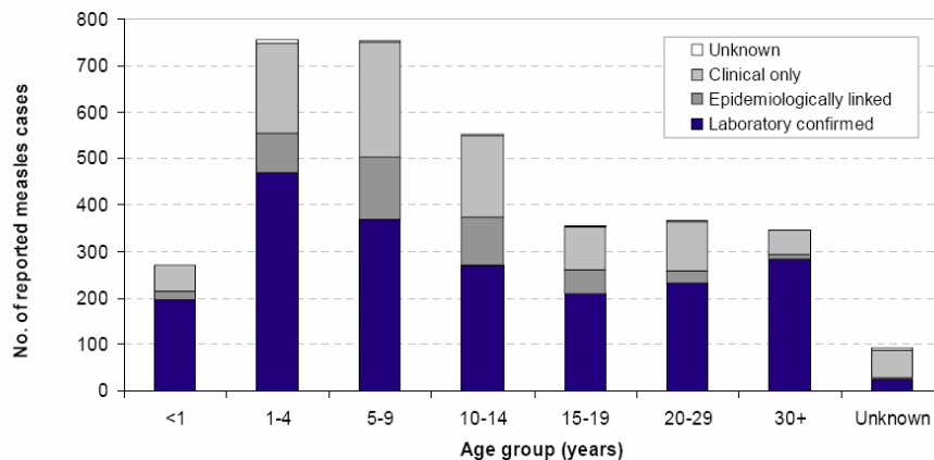
Figure 2. Reported measles cases by age group and confirmation status in all reporting countries, 2007 (n=3,842)
