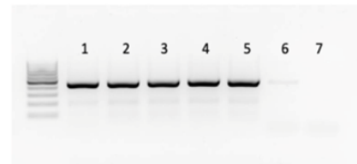
GAPDH
